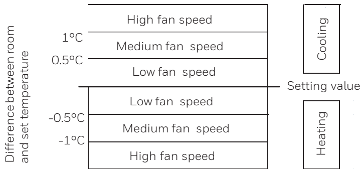
Figure 1. Automatic Fan Speed Control Algorithm
